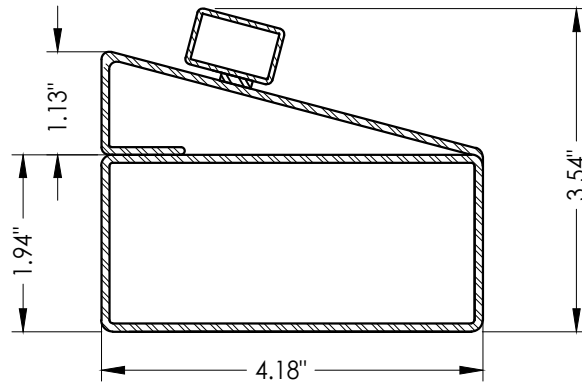
39 SIDELITE BOTTOM RAIL Operable
