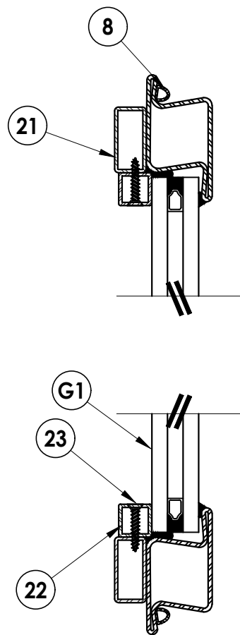
2 VERTICAL CROSS SECTION
