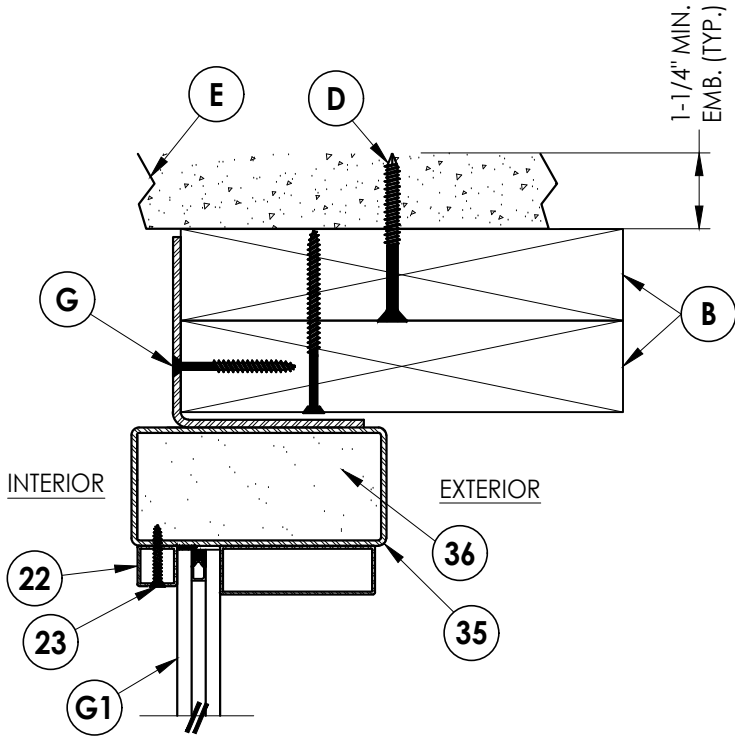
2 VERTICAL CROSS SECTION 5 Outswing shown - inswing also approved
