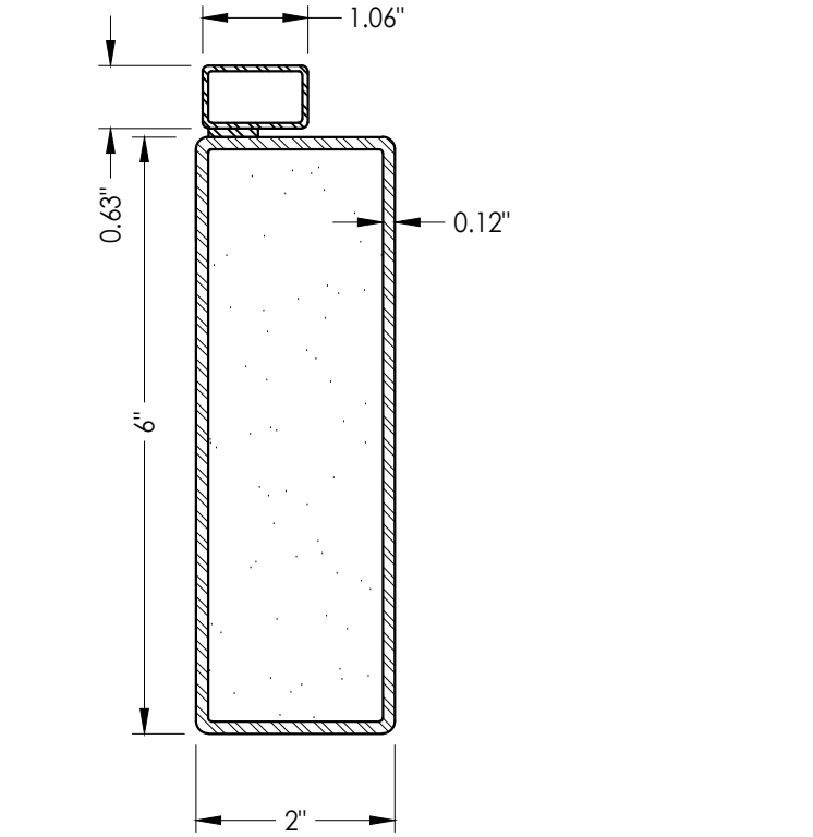
18 TOP, BOTTOM RAIL Foam filled
