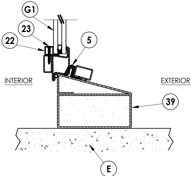
5 VERTICAL CROSS SECTION 5 Outswing shown - inswing also approved
