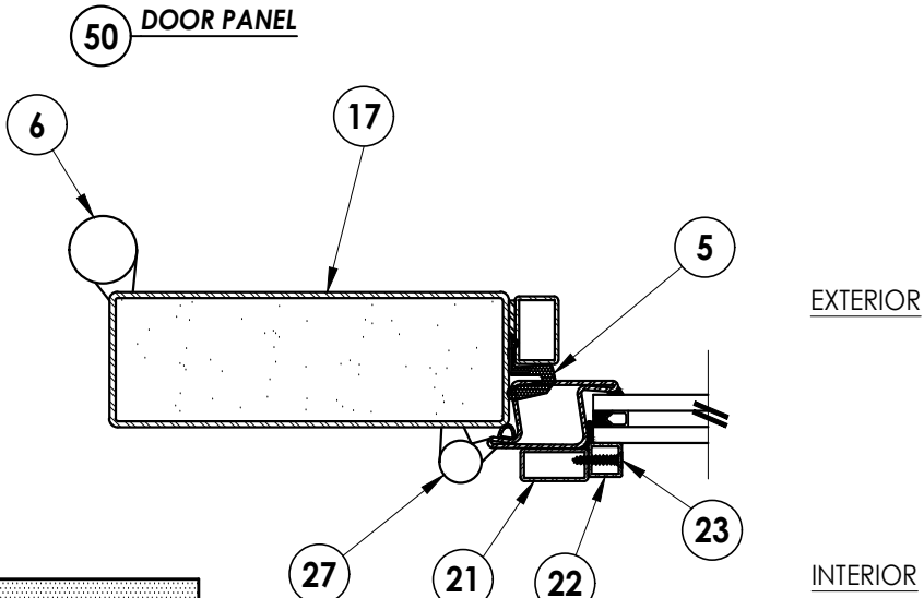
1/2 HORIZONTAL CROSS SECTION
