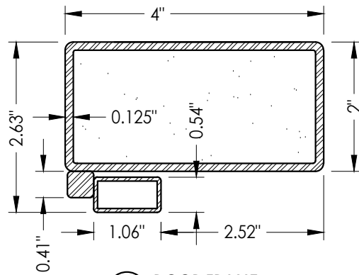
35 DOOR FRAME Foam filled
