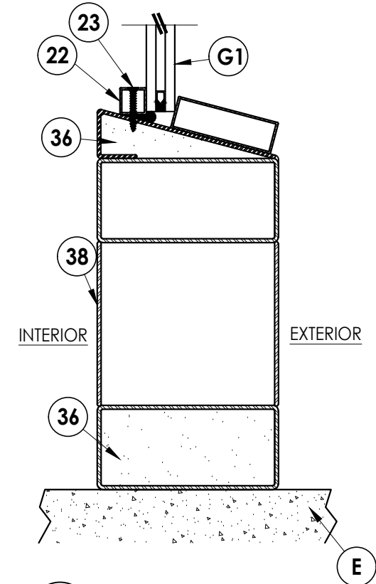
1 VERTICAL CROSS SECTION 5 Outswing shown - inswing also approved
