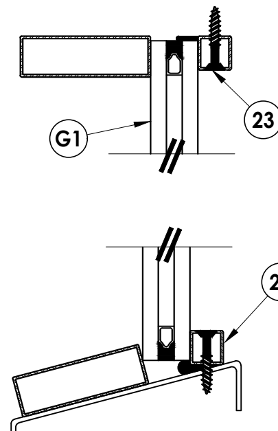
4 VERTICAL CROSS SECTION
