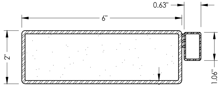
18 TOP, BOTTOM RAIL Foam filled
