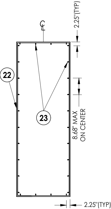
GLASS STOP ANCHORING
